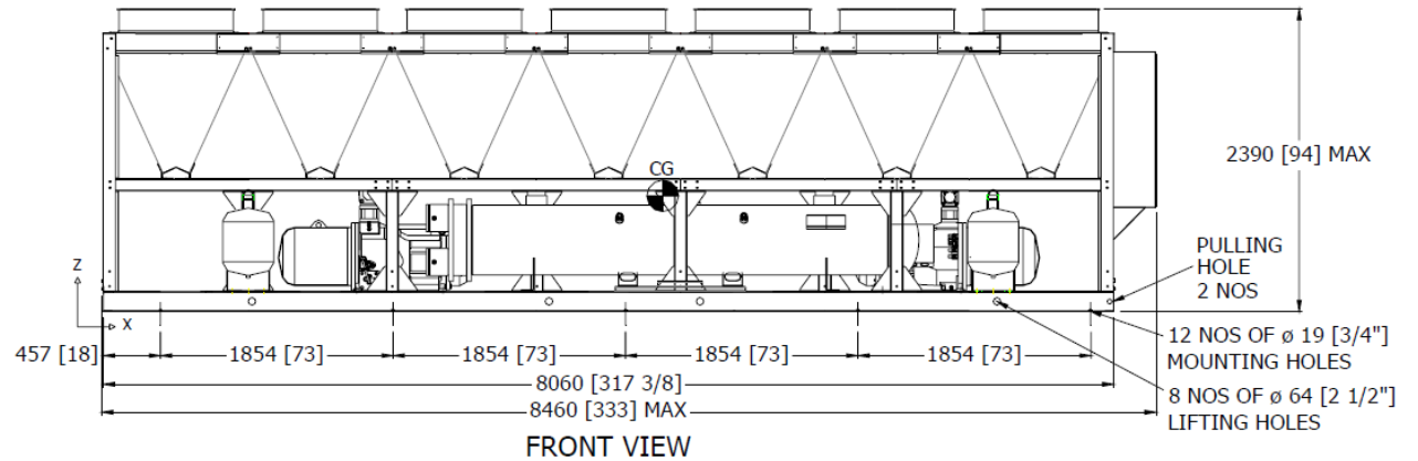
FRONT VIEW
