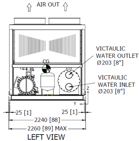
LEFT VIEW
