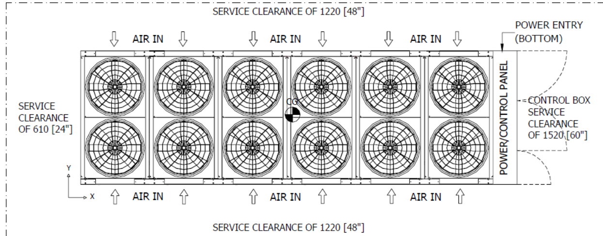
TOP VIEW
