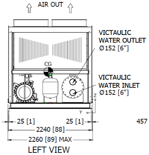
LEFT VIEW
