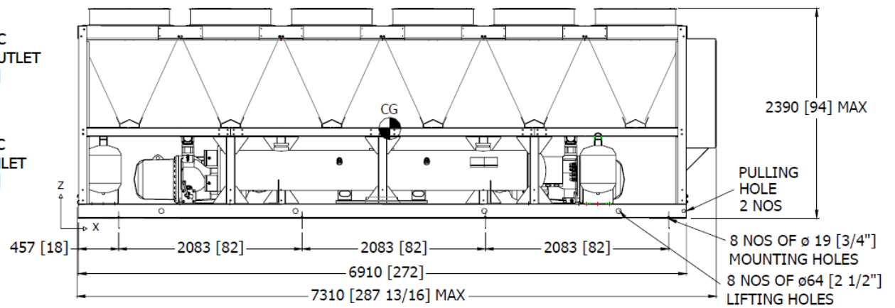
FRONT VIEW
