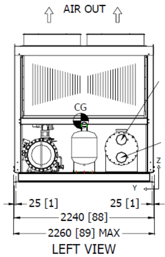
LEFT VIEW
