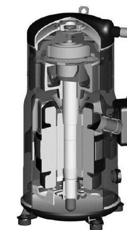
SCROLL COMPRESSOR
