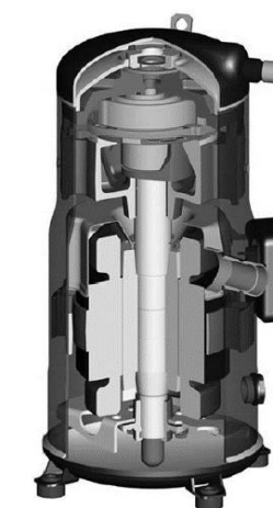
SCROLL COMPRESSOR
